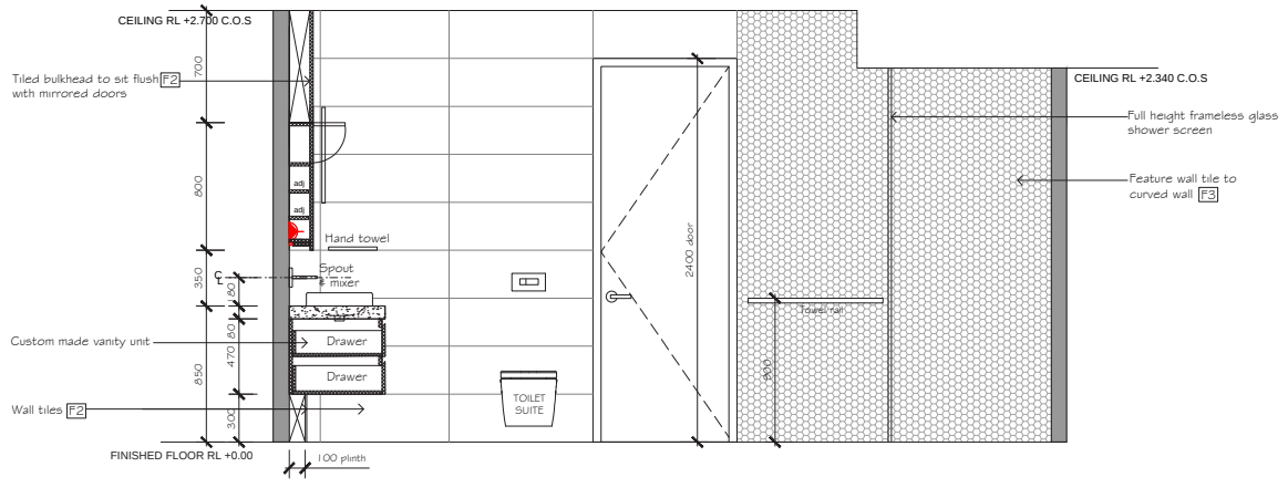
01 ELEVATION 1 SCALE 1:25
