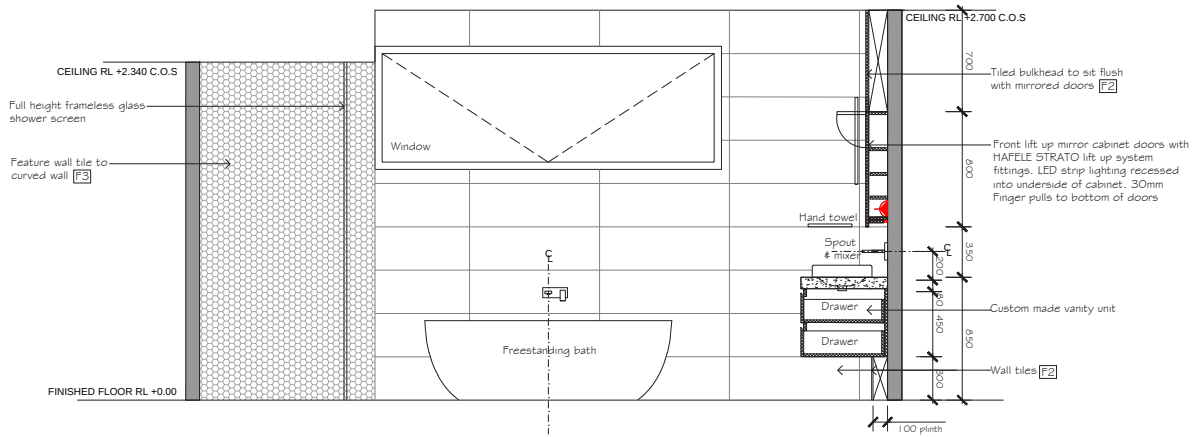
03 ELEVATION 3 SCALE 1:25
